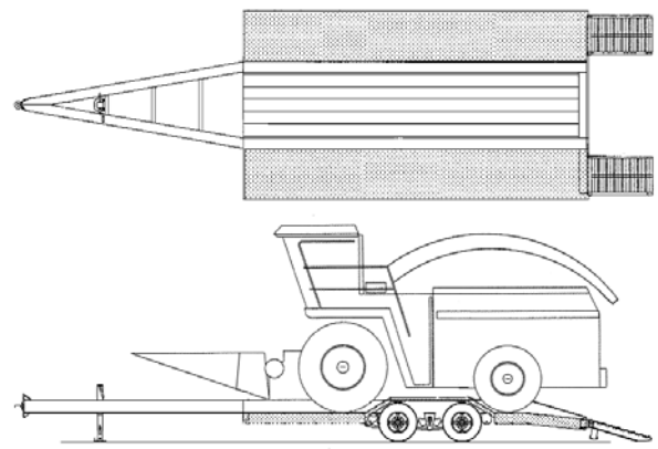
Chopper/Sprayer Trailer loaded with John Deere Chopper
