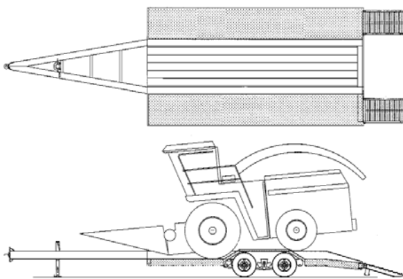
Chopper/Sprayer Trailer loaded with New Holland Chopper
