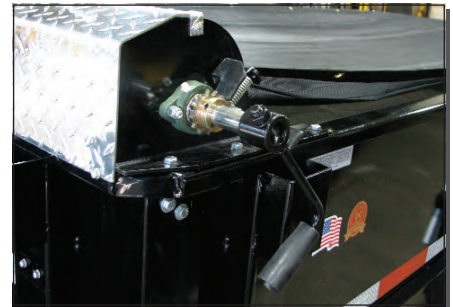
Shown Above: Self-Locking Ratchet system with spring release.
