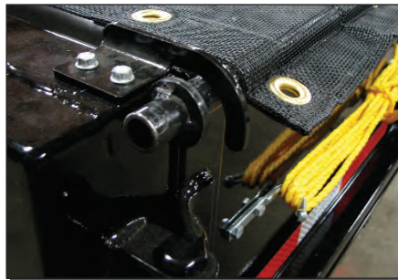
Shown Above: Tarp hook attachment area, keeps the Tarp System Bar in place for transport.
