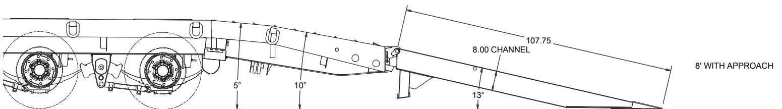
6' Double Incline Beavertail with 8' Air Ramps, with Approach
