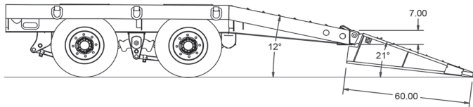
5' Beavertail w / 5' Flip-Over Ramp *Standard
