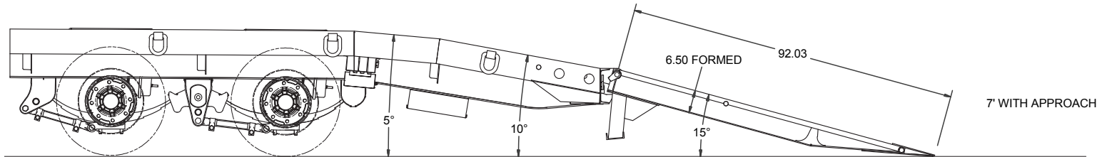
6' Double Incline Beavertail with 7' Air Ramps, with Approach
