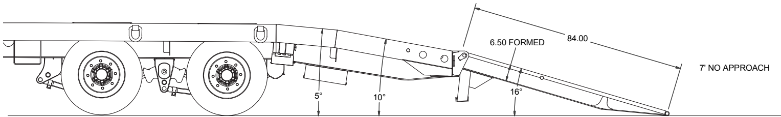
6' Double Incline Beavertail with 7' Air Ramps, No Approach
