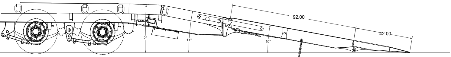
6' Double Incline Beavertail with 11' Air Bi-Fold Ramps
